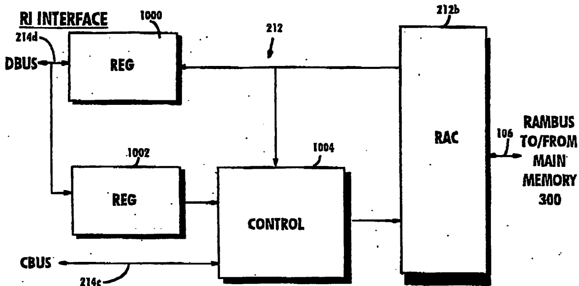
Fig. 36 EXAMPLE MEMORY INTERFACE
